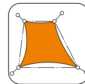
Trapez
